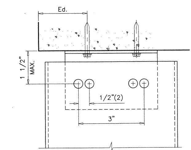
LOCATION OF SCREWS CONNECTING ANGLES TO TUBES
